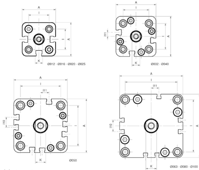
Model ASM, ASEM, ADM, ADMP
