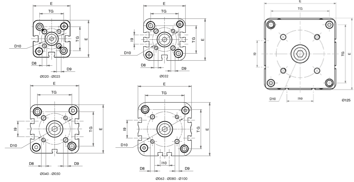
Model PDMA en PDMPA
