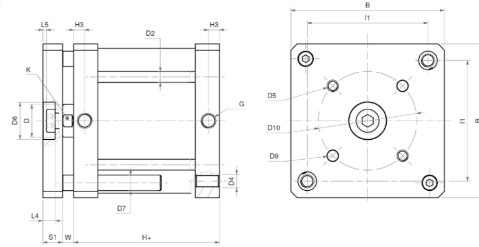
Model KDA, KDMA
