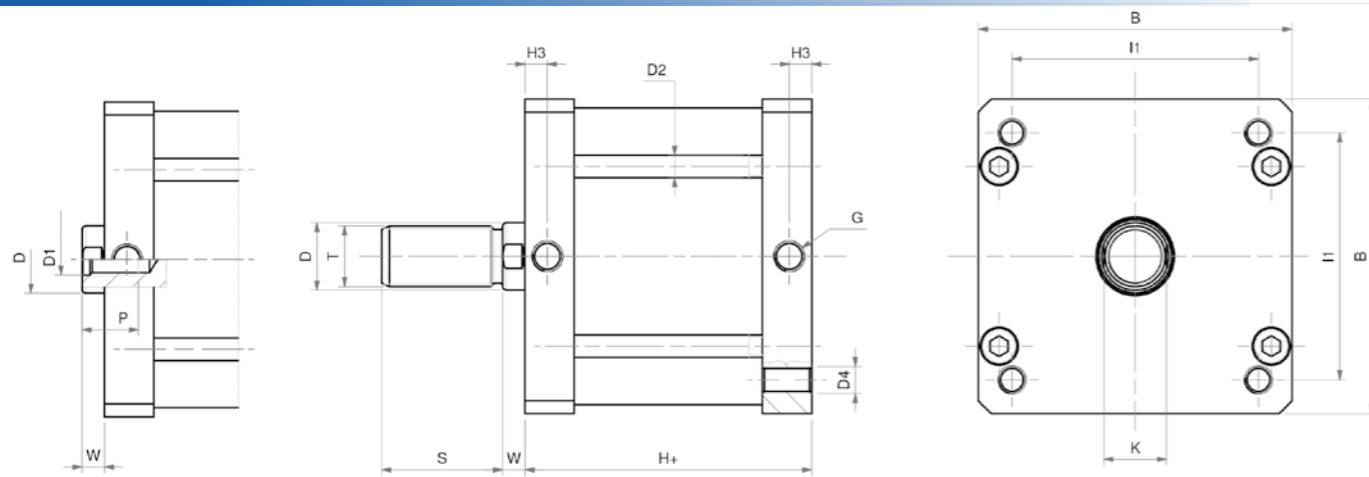
Model KS, KSM, KD, KDM, KDP, KDMP
