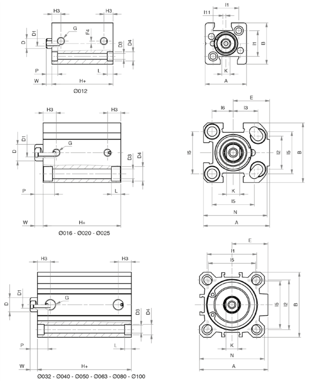
Model FSR, FSM, FDR, FDM
