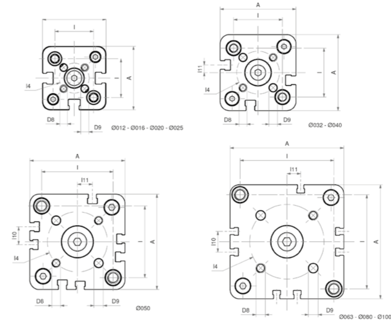
Model ADMA, ADMPA
