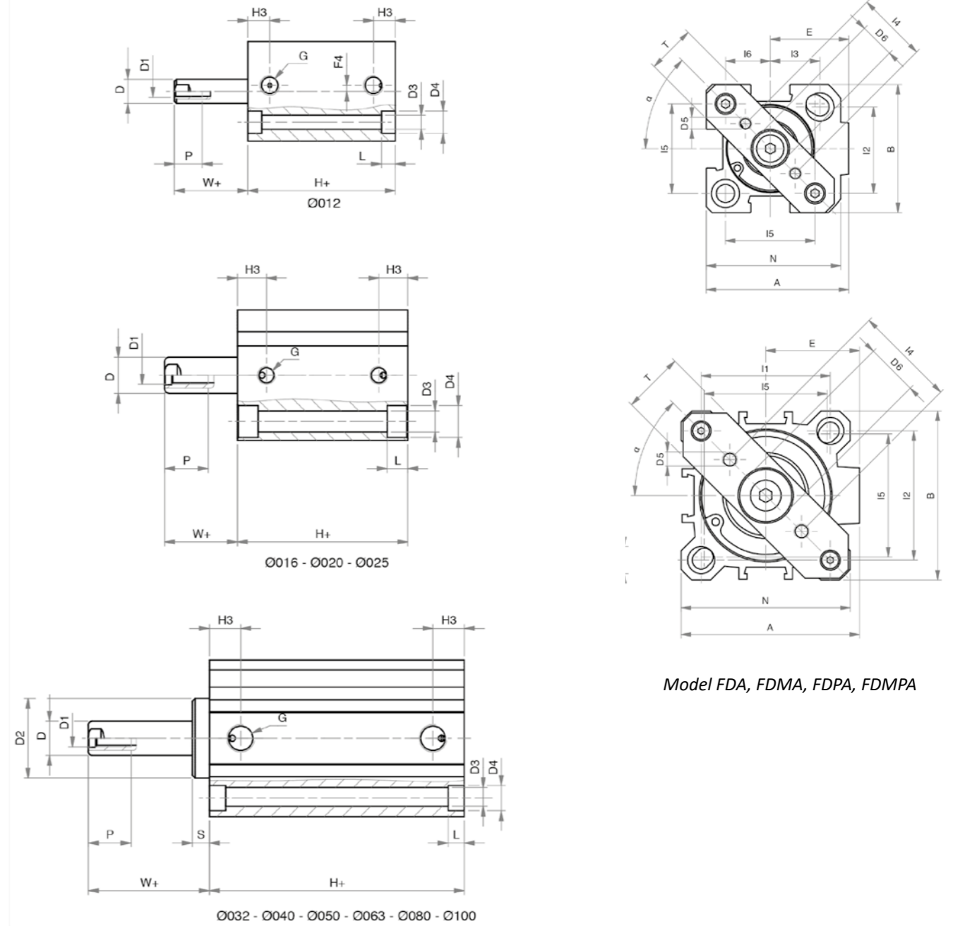
Model FSE, FSEM
