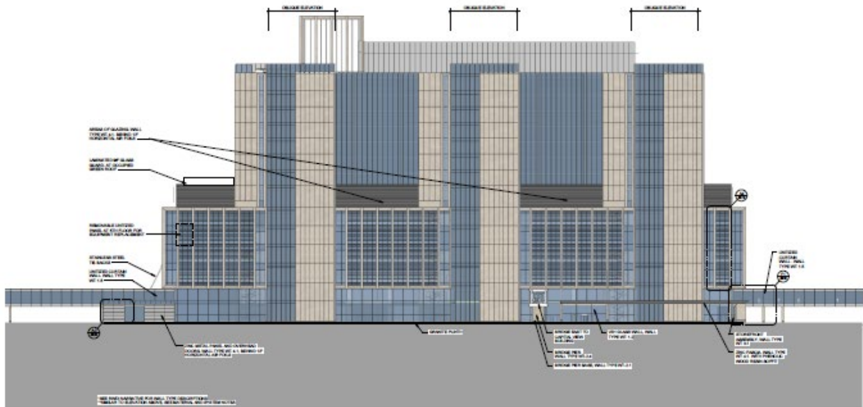
EAST EXTERIOR ELEVATION 1/8" = 1'-0"
