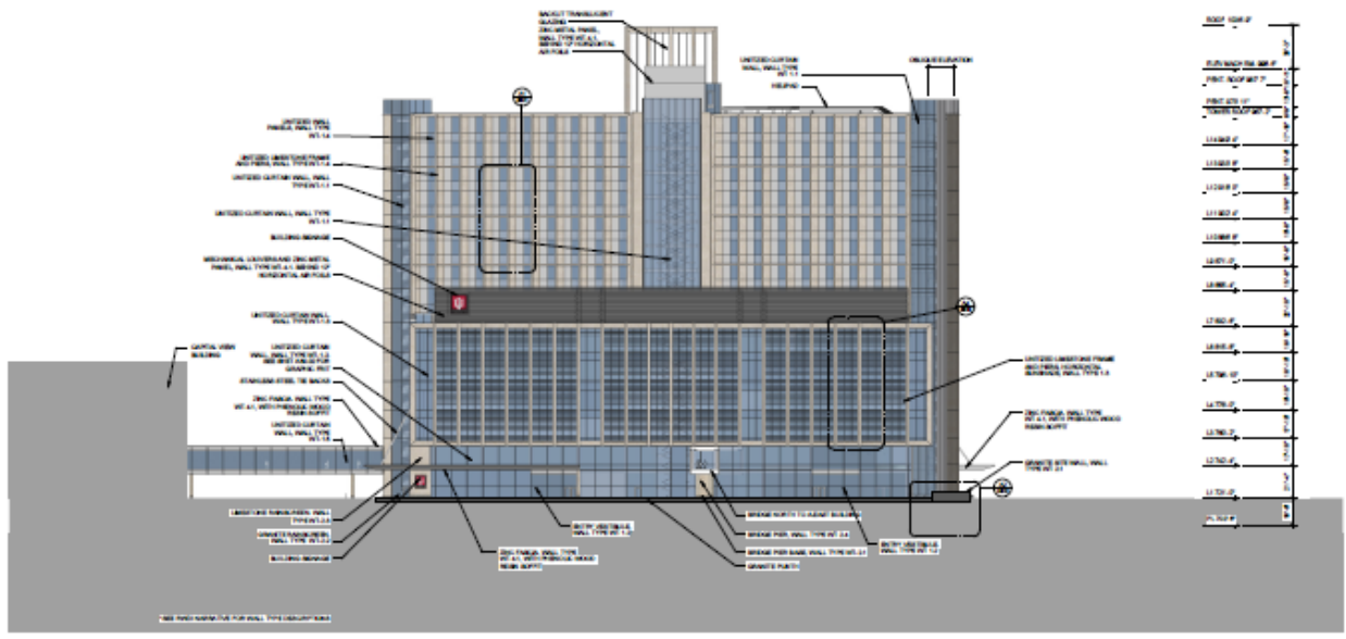
NORTH EXTERIOR ELEVATION 04/21/18
