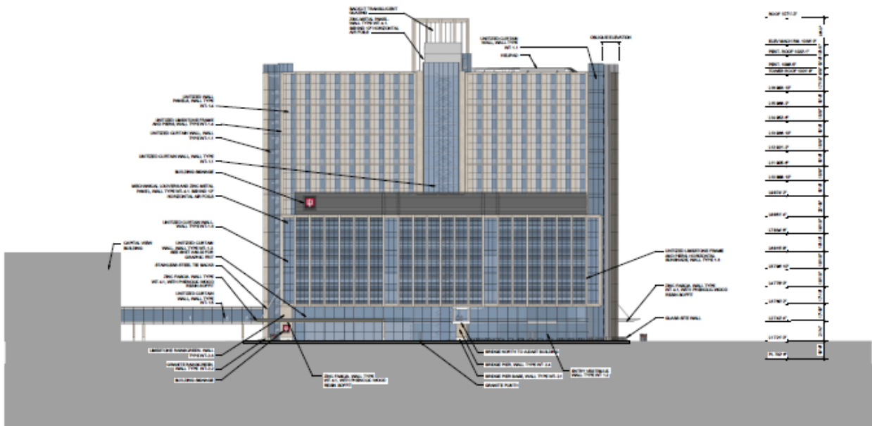
NORTH EXTERIOR ELEVATION 1/32" = 1' 0"
