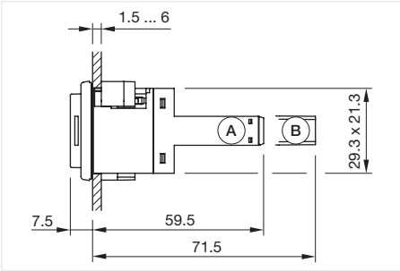
Dimensions [mm] A = Screw terminal B = Plug-in terminal 6.3 mm x 0.8 mm
