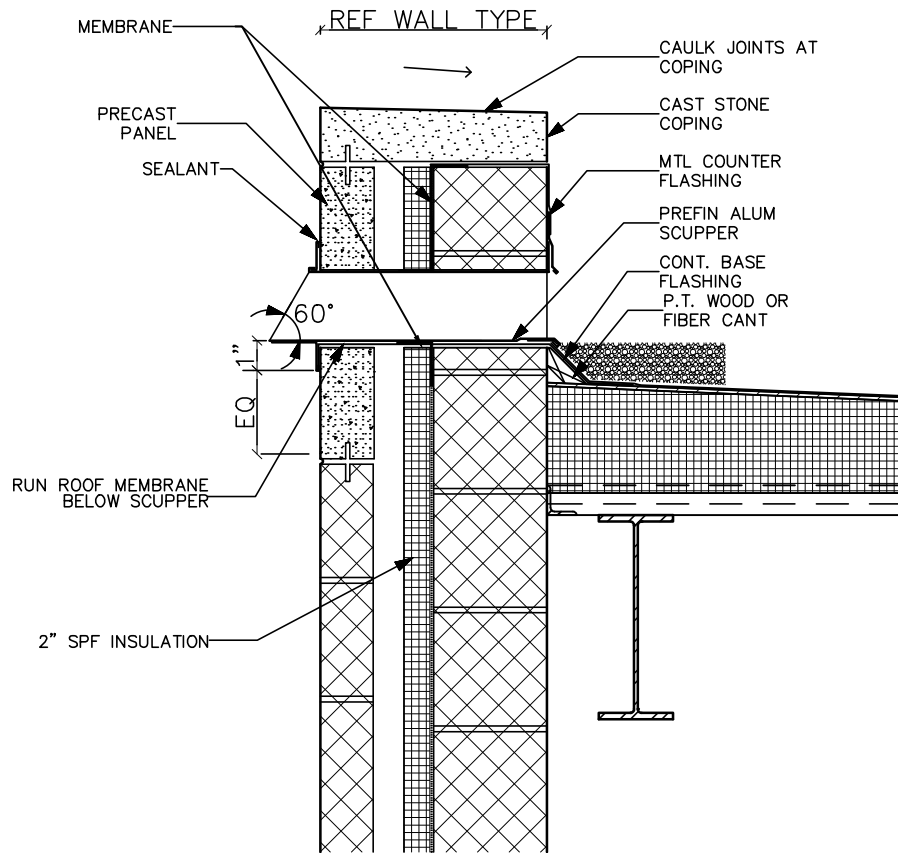
1 PARAPET / OVERFLOW SCUPPER WALL 1"=1' - 0"
