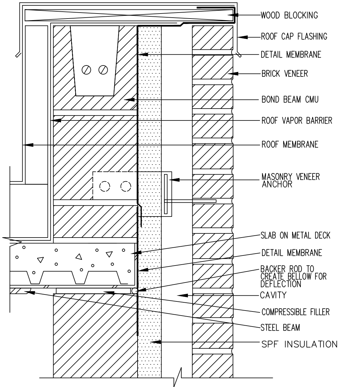
Roof Detail Parapet 1 CMU
