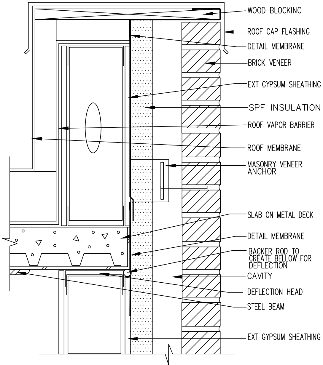
Roof Detail 2 Parapet
