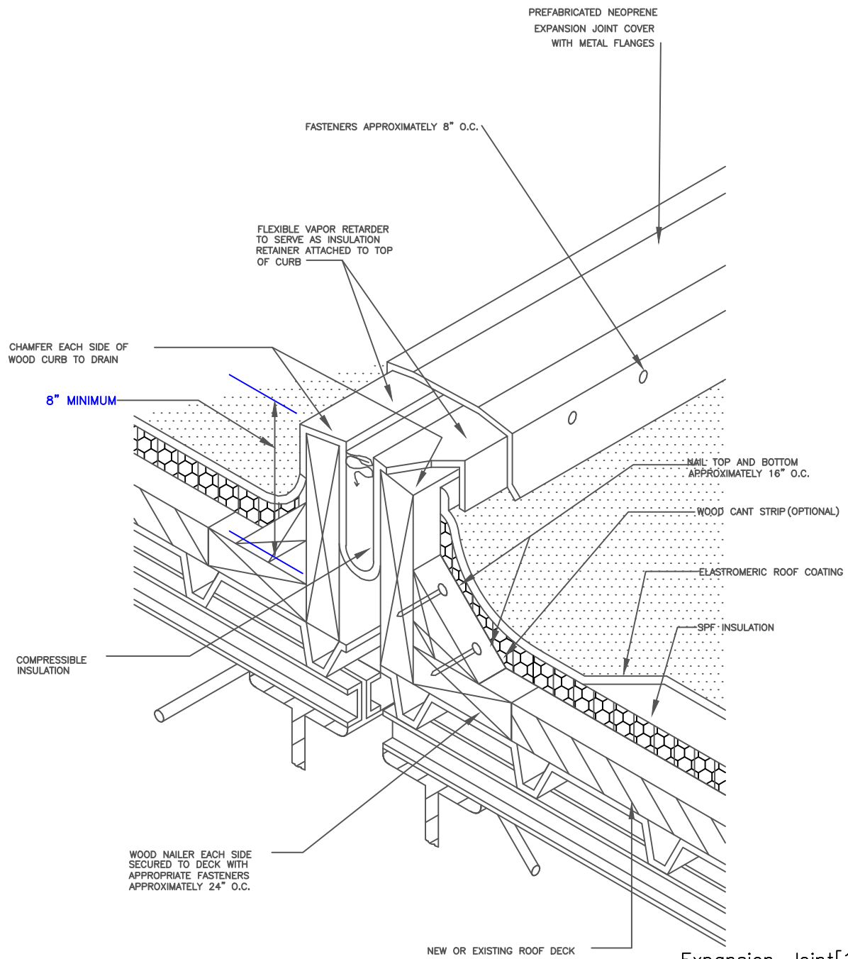
Expansion_Joint[1]
