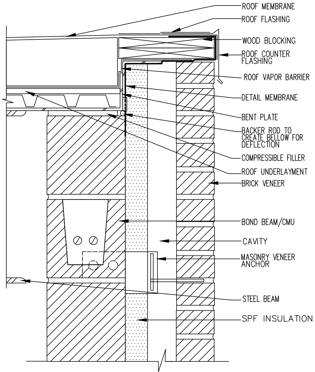
Roof Detail 2 CMU
