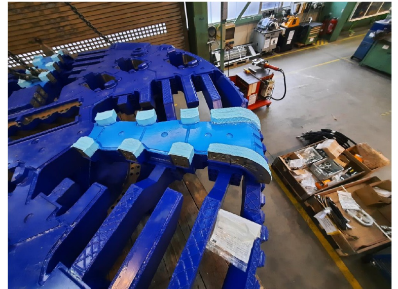
Cutterhead
