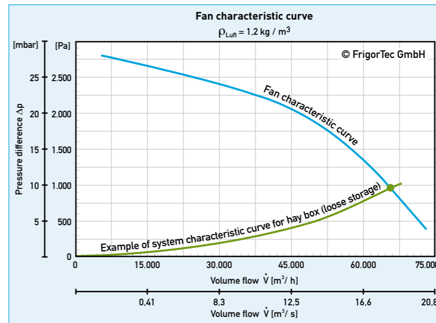
20 Characteristic curve of an AGRIFRIGOR™ fan
