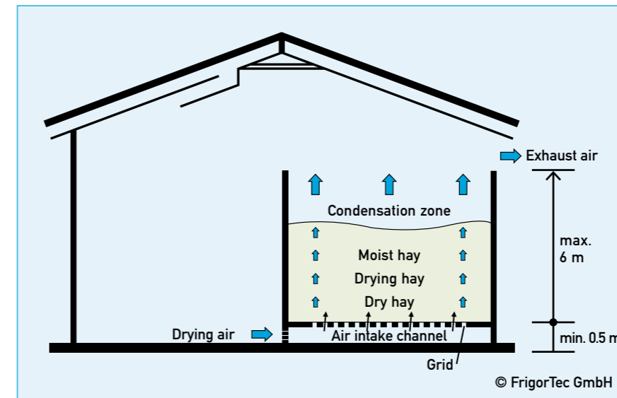
25 Drying process in the hay box
