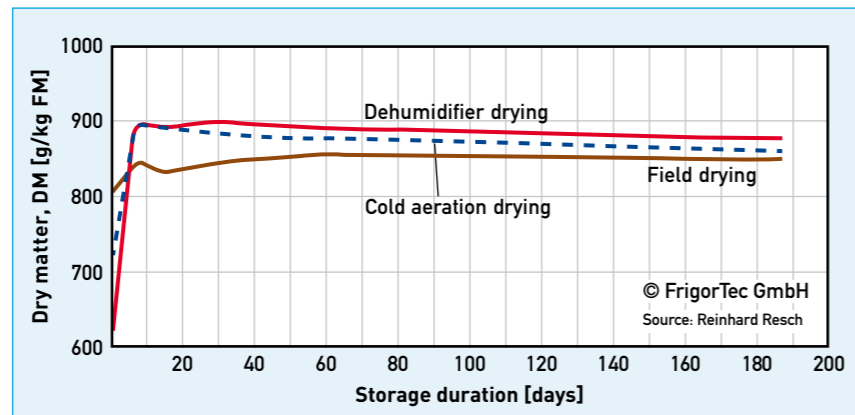
3 Influence of different drying methods on the dry matter content DM (2)
