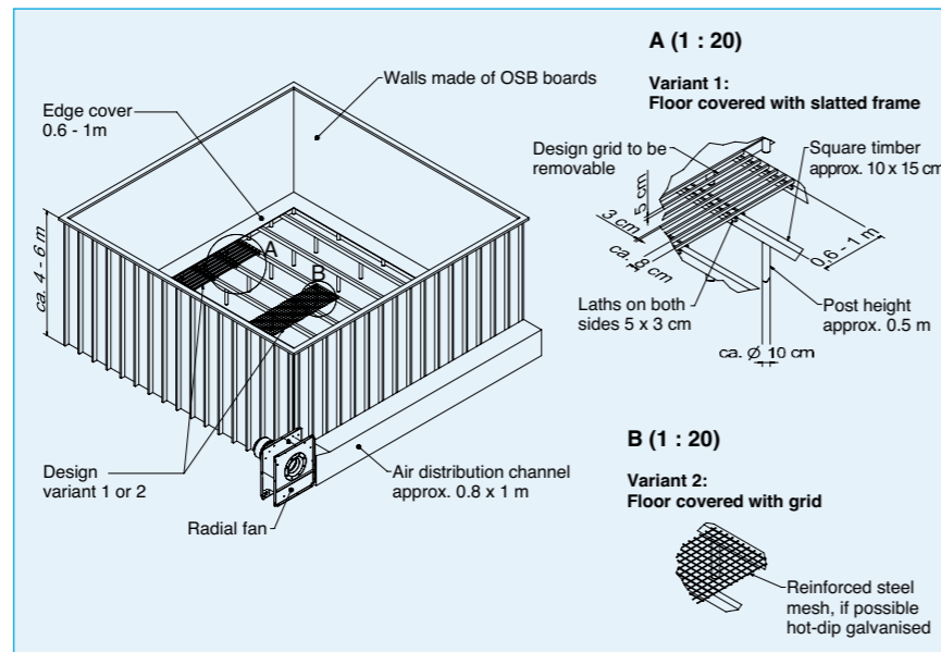
22 Design drawing of hay box with slats/grid
