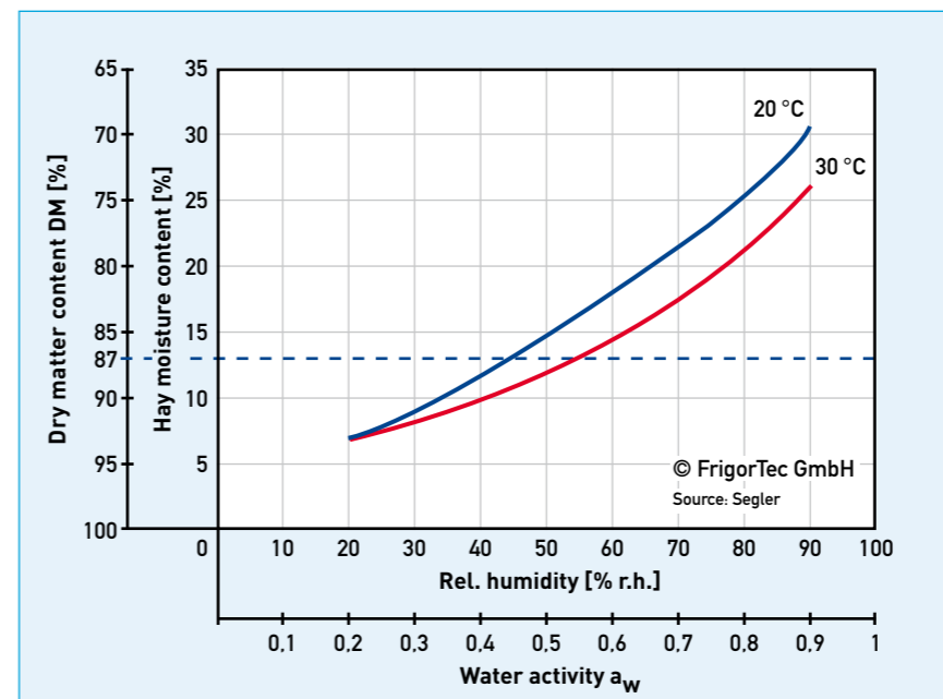
21 Sorption isotherms of hay
