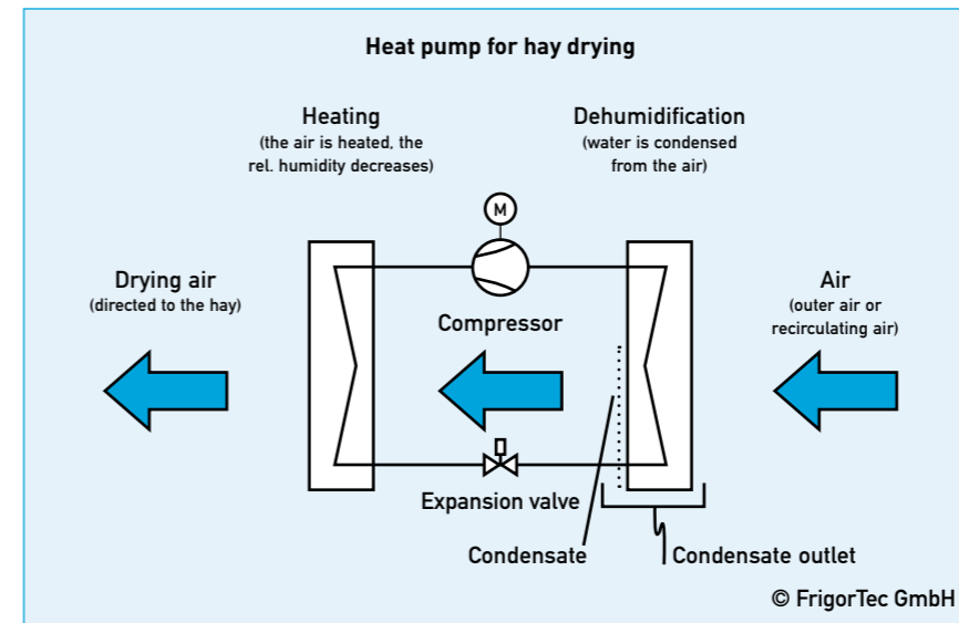
12 Heat pump process for air dehumidification
