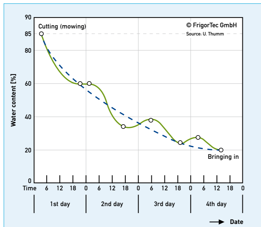
1 Moisture development during field drying
