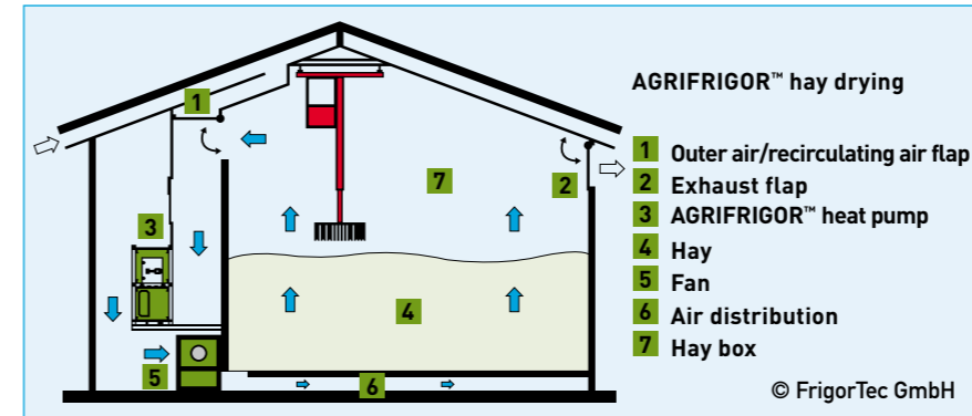
11 AGRIFRIGOR™ process of drying hay by heat pump or dehumidifier
