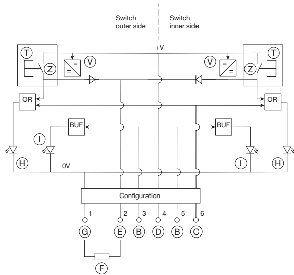
Wiring diagram 1
