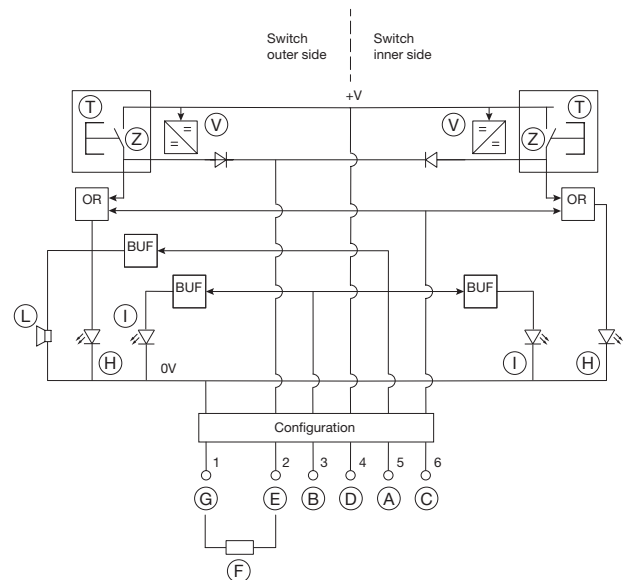
Wiring diagram 4
