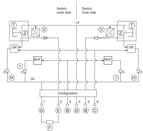
Wiring diagram 2
