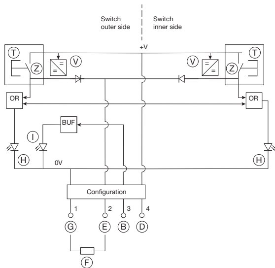
Wiring diagram 1
